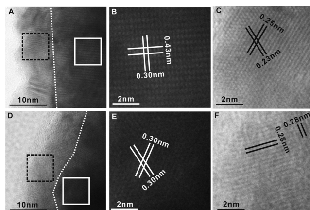
Figure 3. A) High-resolution TEM image of CuO/c - Cu_2O in Cu_2O [1\bar{1}0] view. B) Enlarged high-resolution TEM image of the inner region of CuO/c - Cu_2O indicated by the solid white square in (A). C) Enlarged high-resolution TEM image of the surface region of CuO/c - Cu_2O indicated by the dash black square in (A). D) High-resolution TEM image of CuO/o - Cu_2O in Cu_2O [1\bar{1}1] view. E) Enlarged high-resolution TEM image of the inner region of CuO/o - Cu_2O indicated by the solid white square in (D). F) Enlarged high-resolution TEM image of the surface region of CuO/o - Cu_2O indicated by the dash black square in (D). The dashed white lines in (A) and (D) indicate the CuO - Cu_2O boundary in CuO/c - Cu_2O and CuO/o - Cu_2O , respectively.
